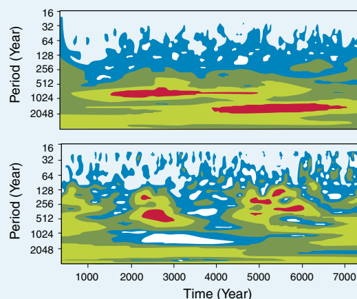
Periodicity of oaks (top) and 14 C production (bottom).
